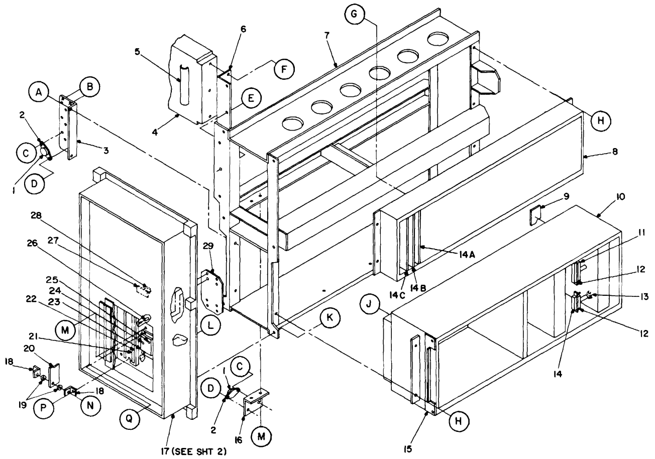
Figure 60. Test assy plug-in unit, wired, 10281449 (Sheet 1 of 4).
