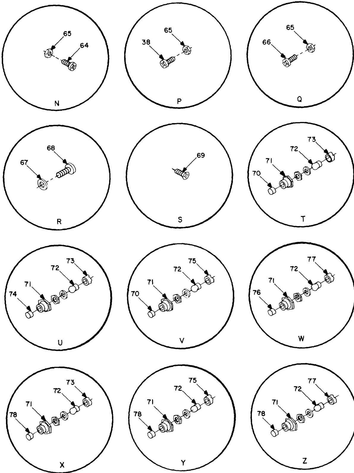
Figure 60. Test assembly plug-in unit, wired, 10281449 (Sheet 4 of 4).
