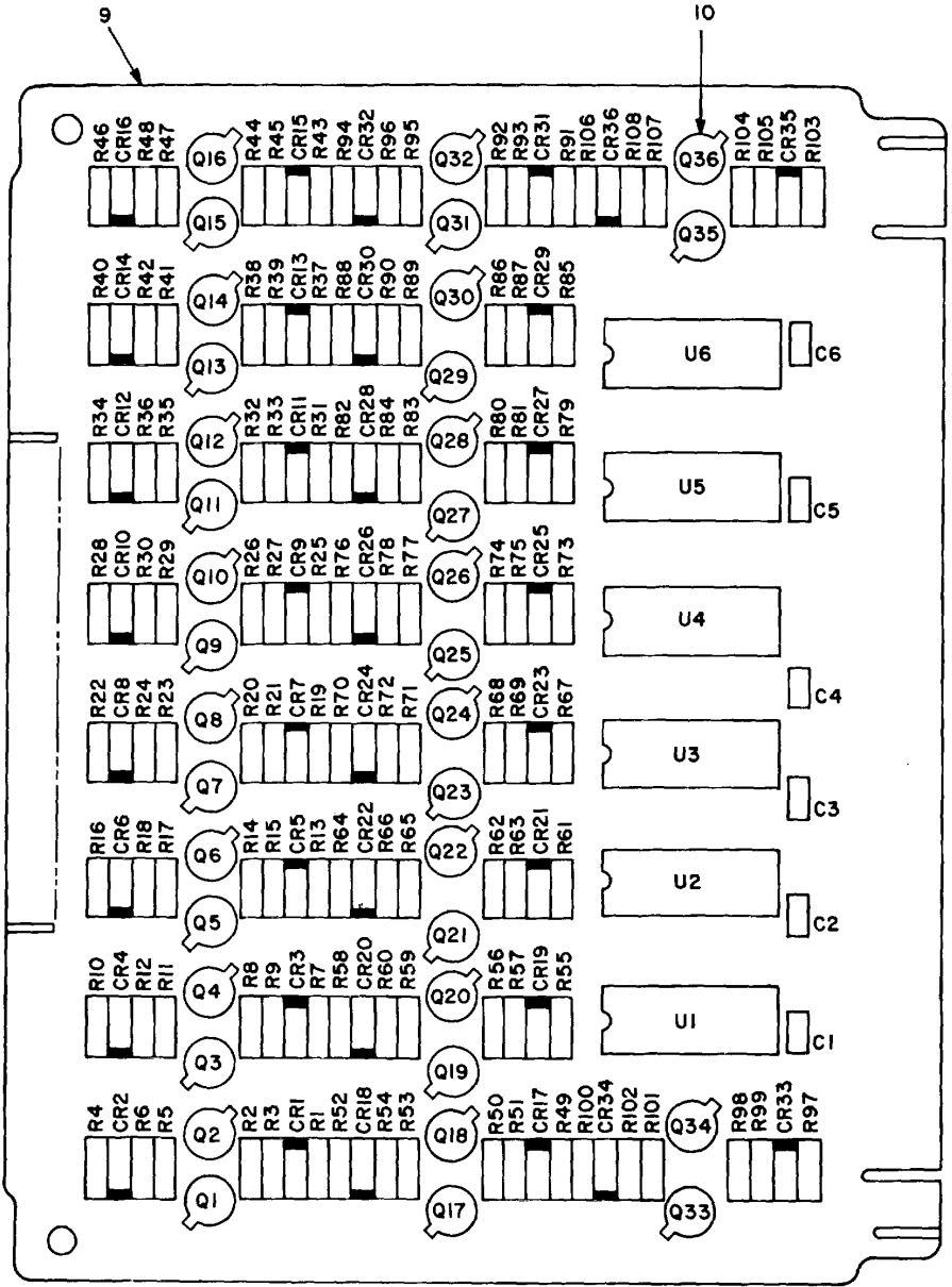
Figure 18. Circuit card assy, 10282752 (Sheet 1 of 2).
