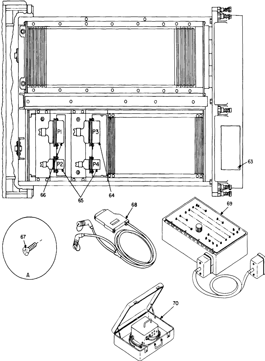
Figure 1. Module test set (Sheet 5 of 5).
