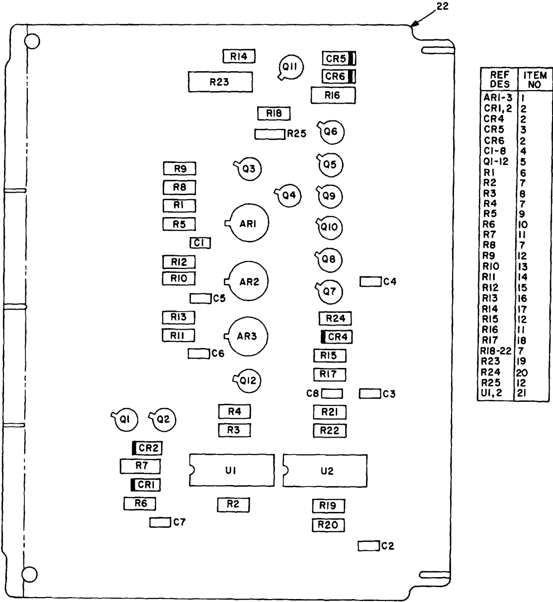
Figure 14. Circuit card assy, 10281785.
