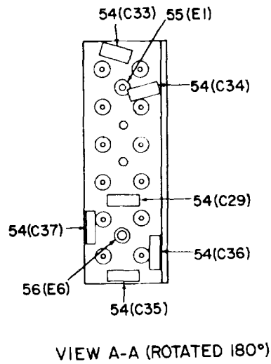
Figure 58. DC/DC converter PS1, 126650-102 (Sheet 2 of 3)
