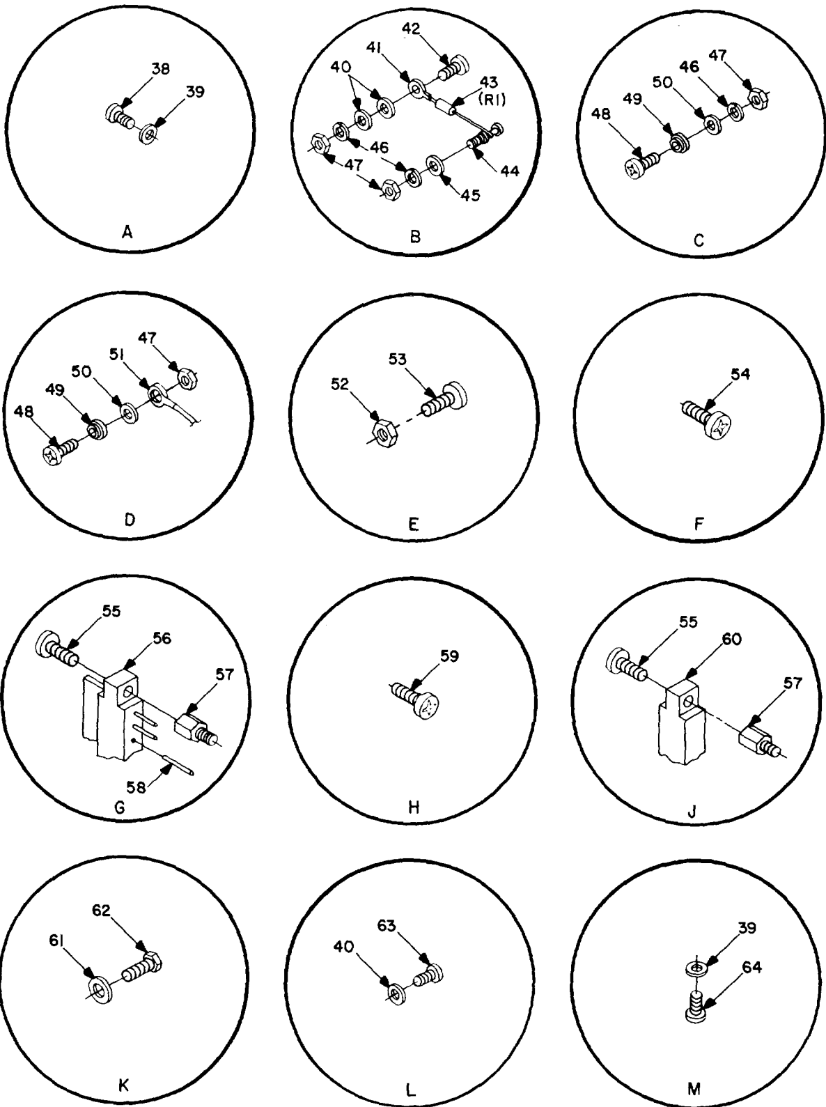
Figure 60. Test assy plug-in unit, wired, 10281449 (Sheet 3 of 4).
